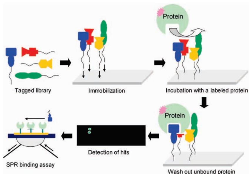
FIGURE 6. Advantageous immobilization of the tagged library with intrinsic tags on small molecule microarrays.
